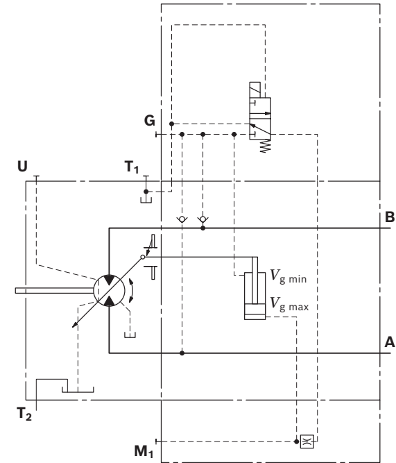
▼ Circuit diagram EZ5, EZ6 (negative control) Size 28 and 140 to 215
