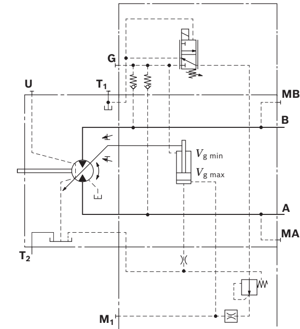
▼ Circuit diagram EZ5, EZ6 (negative control) Size 280
